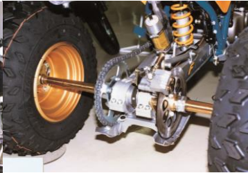
Wheel Axis Sprocket Stopper
